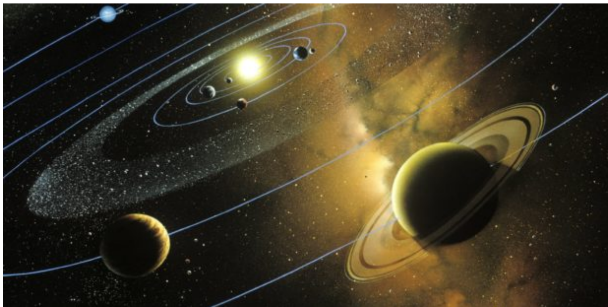
Solar System orbits, artwork
